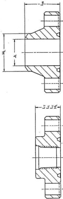
Weld Neck Flange
